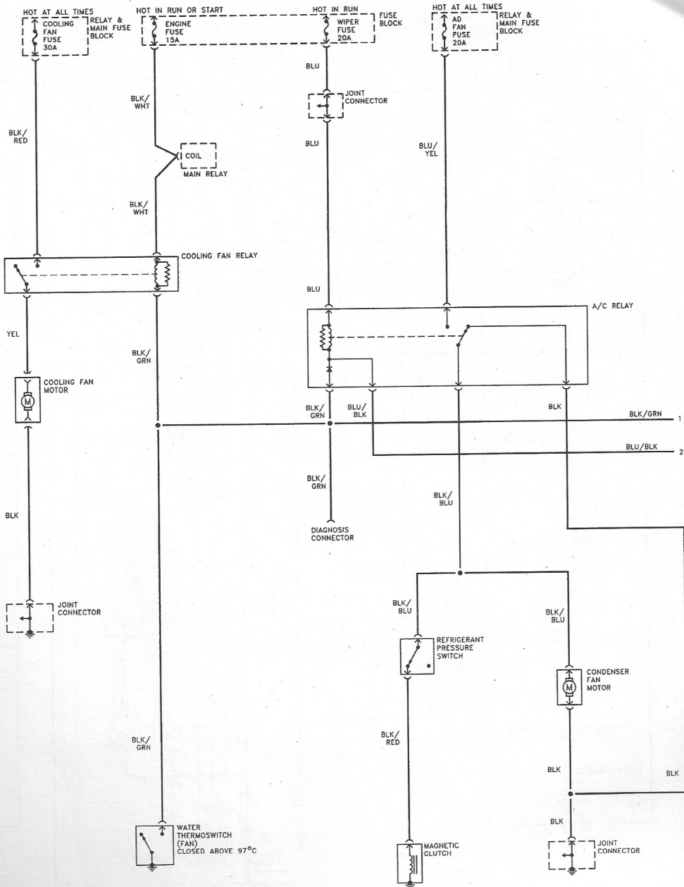
Heating and air conditioning system (includes engine cooling fan system) - 1993 and earlier models (1 of 2)
