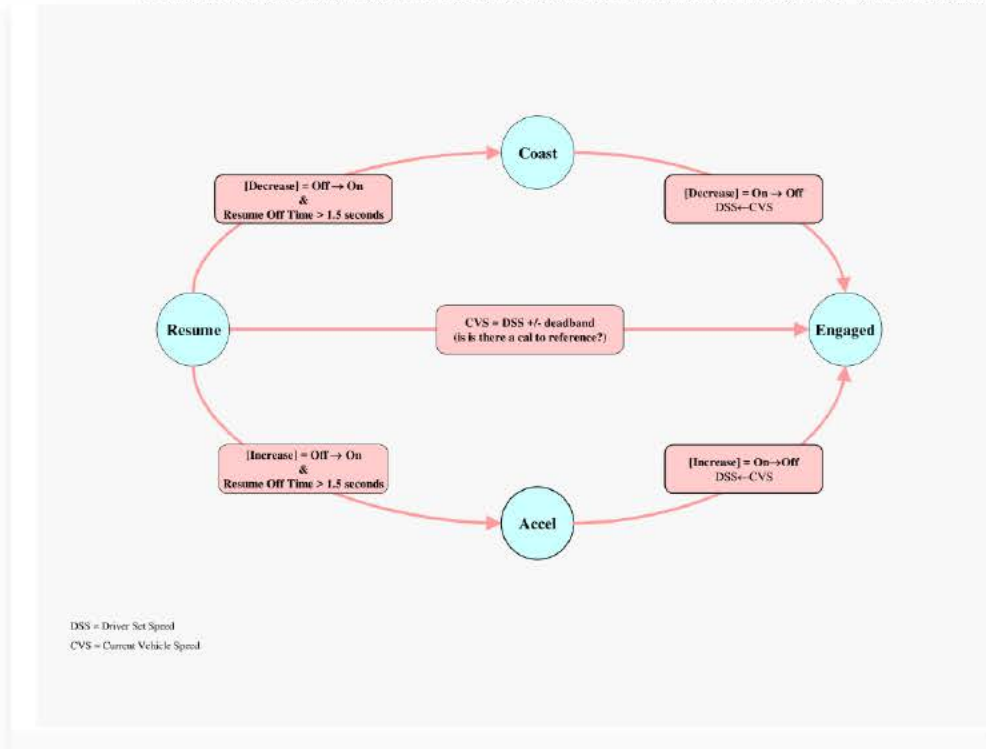
Figure 6: Cruise Control State Diagram
