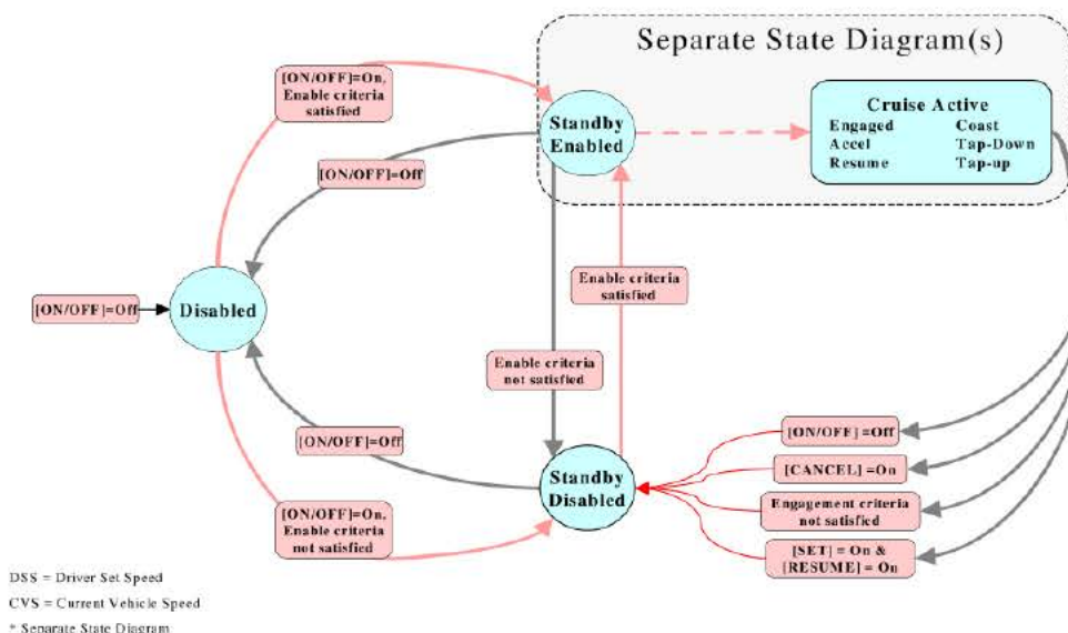
Figure 2: Cruise Control State Diagram (Enabled/Disabled)
